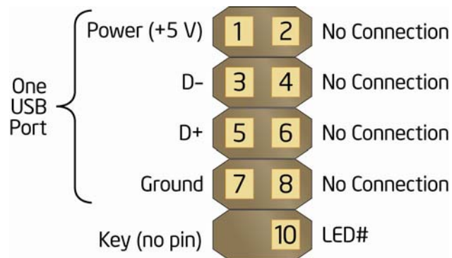
Figure 13. Connection Diagram for Front Panel USB Header with Intel Z- USB Solid-State Drive or Compatible Device Support
