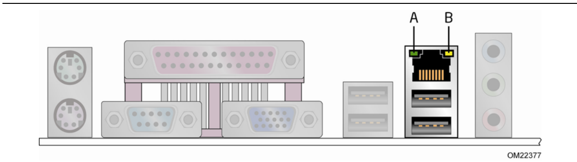
Figure 3. LAN Connector LED Locations
