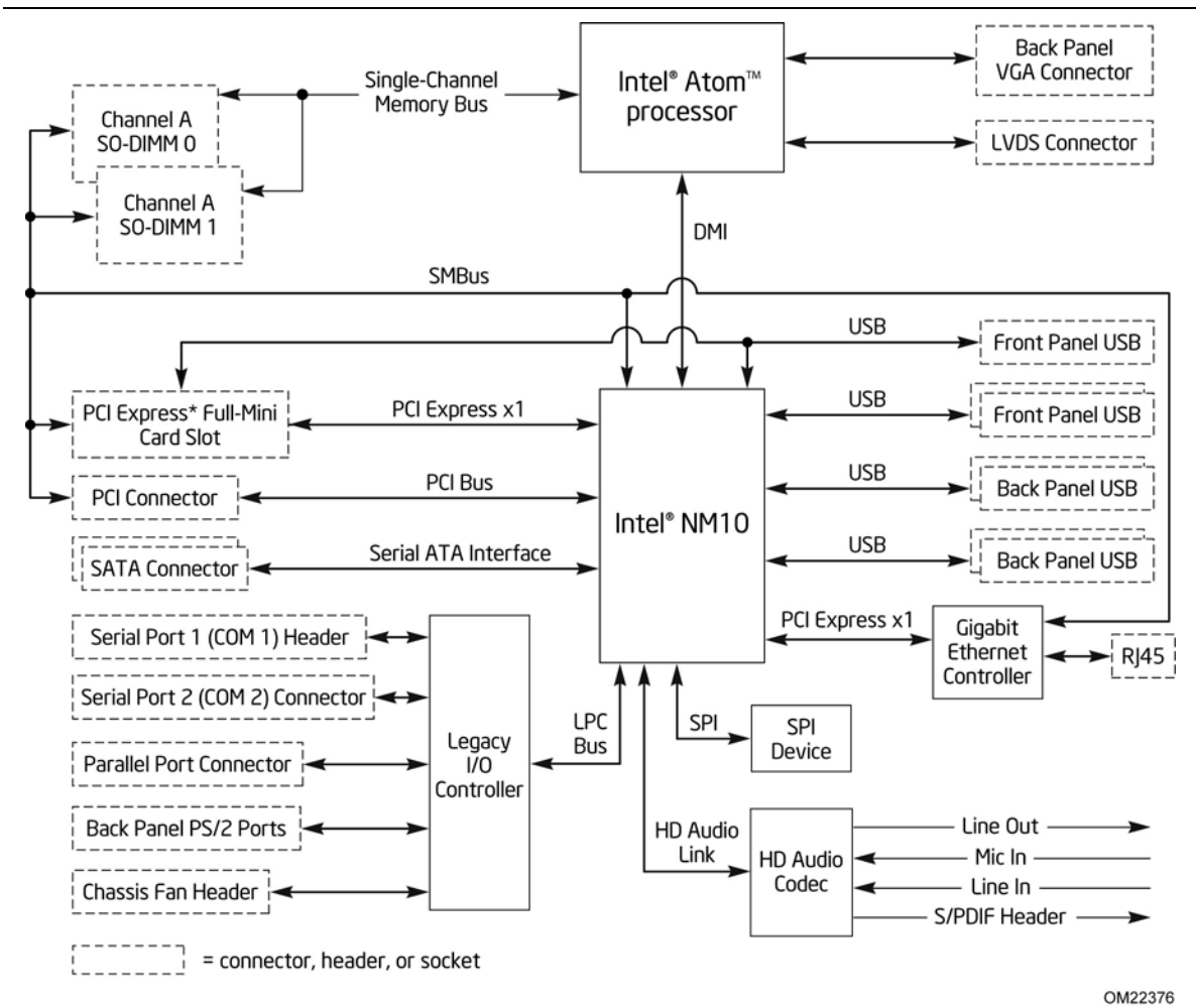
Figure 2. Block Diagram
