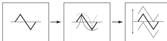
LFO Signal Flow
