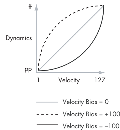
Velocity Bias
